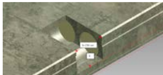
Figur 2: Hammerhovedudsparing
